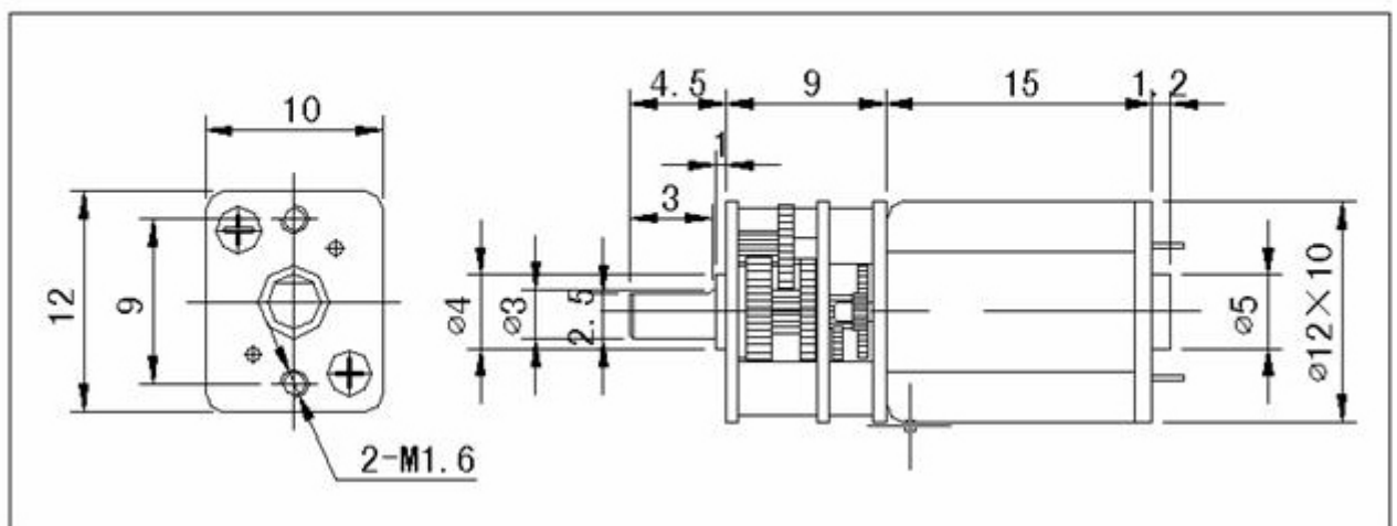
DIMENSIONS(Unit:Millimeter)
