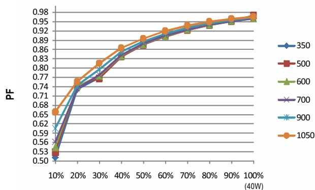
LOAD (277Vac Input)
