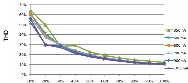
LOAD (277Vac Input)
