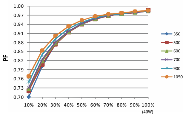
LOAD (230Vac Input)
