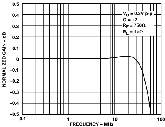
Figure 35. Gain Flatness; V_S = \pm 5\text{ V}
