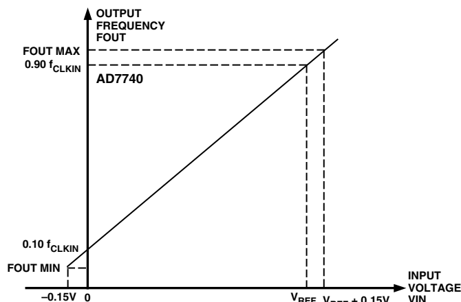
Figure 4. Transfer Function
