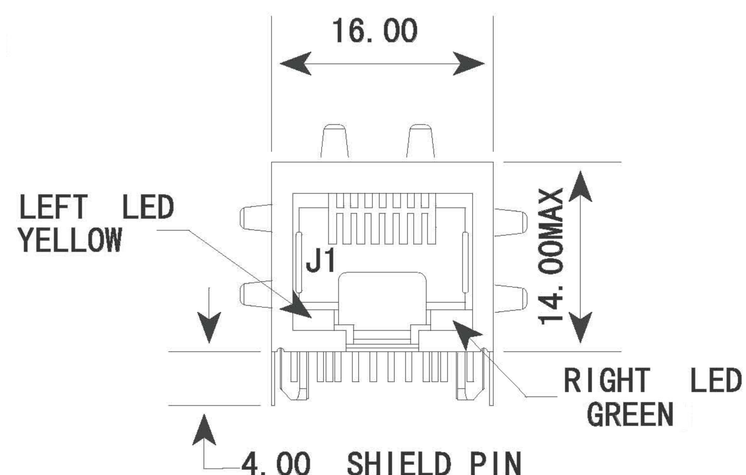
FRONT VIEW
