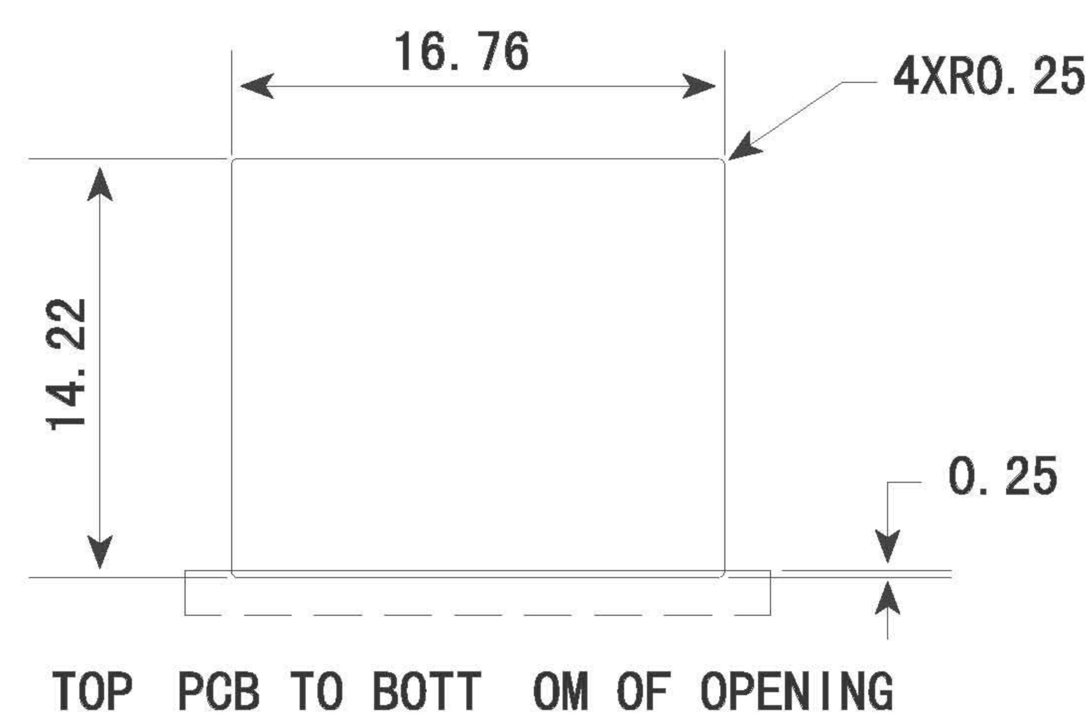
TOP PCB TO BOTT OM OF OPENING
