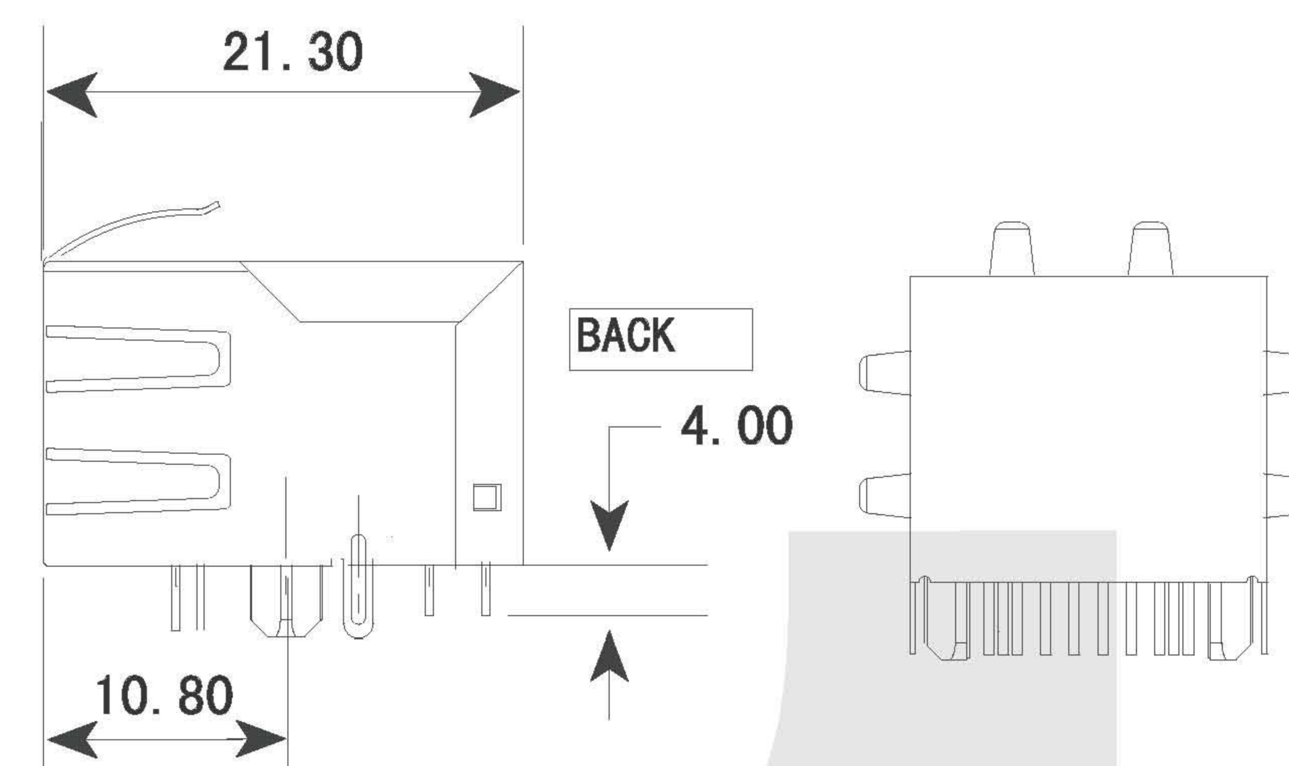
SIDE VIEW
