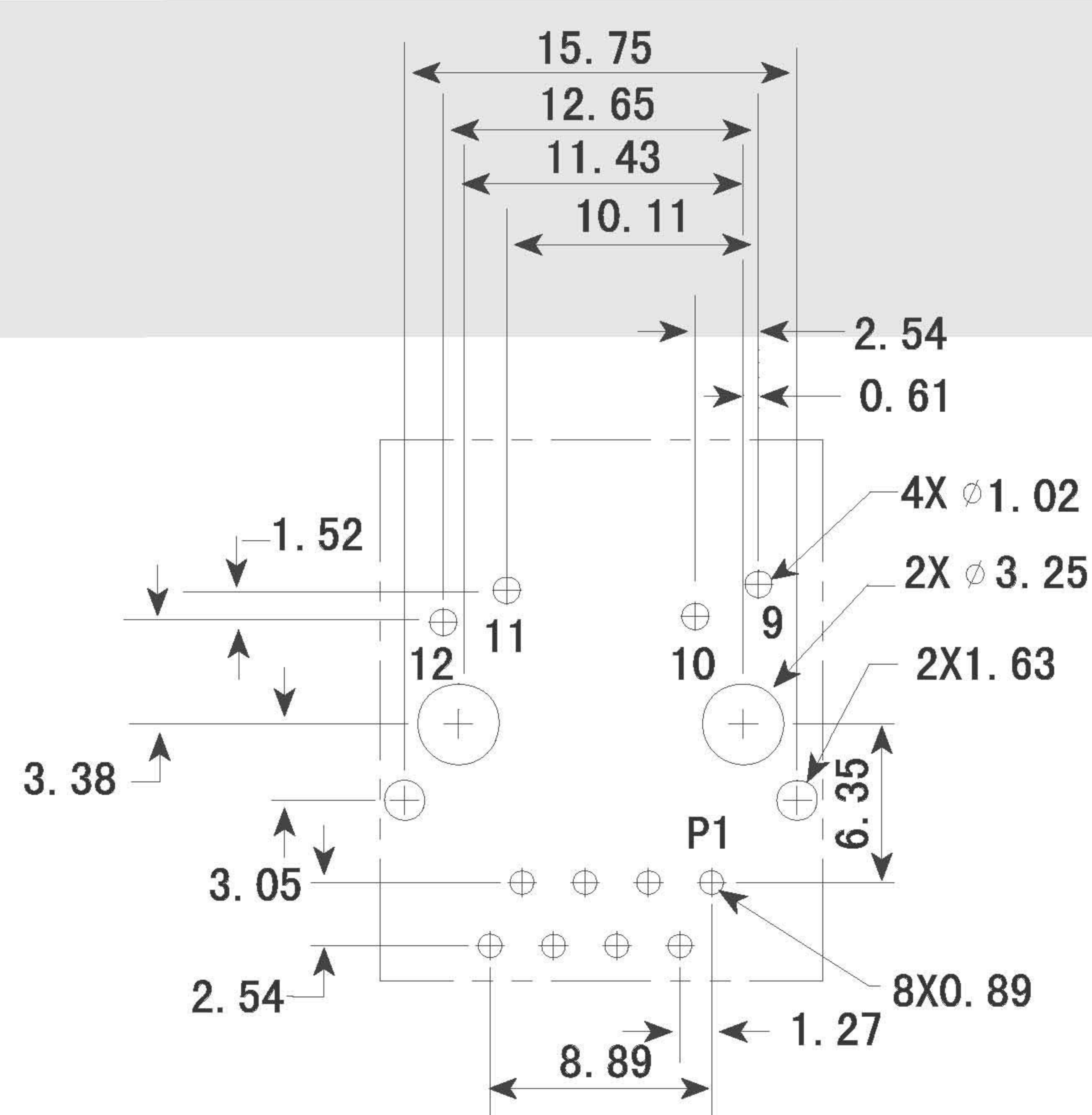
Viewed from PCB Component side
