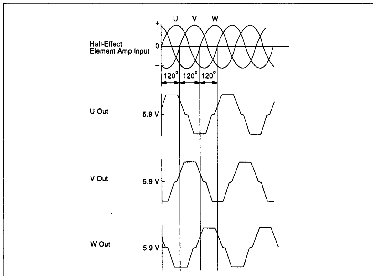
Figure 6 Timing Waveform
