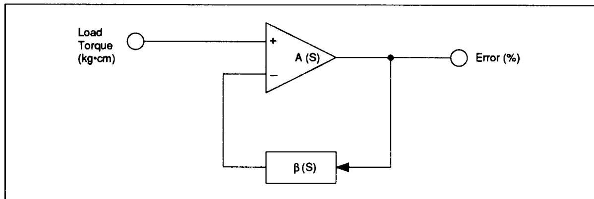
In Figure 1, when A(S) = \frac{K_j}{J \cdot S} \cdot \frac{100}{No} \dots\dots\dots(3) \beta(S) = \frac{K_T}{Z_m(S)} (K_v \cdot G_1(S) \cdot G_2(S) - \frac{K_E \cdot No}{100}) \dots\dots\dots(4) Then Figure 1 can be shown in Figure 2.
