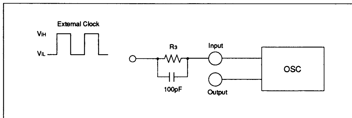
Figure 4 External Clock
