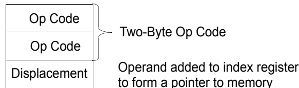
Figure 30. Indexed Addressing Mode
