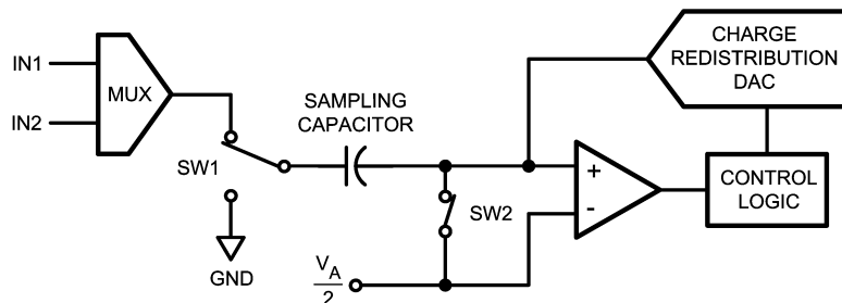
FIGURE 1. ADC122S021 in Track Mode
