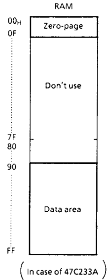
Figure 2. RAM addressing
