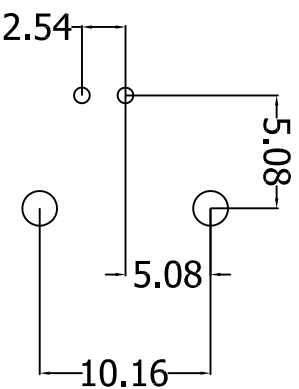
PCB HOLE
