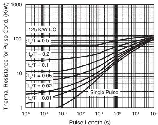
Fig. 8 - Thermal Response
