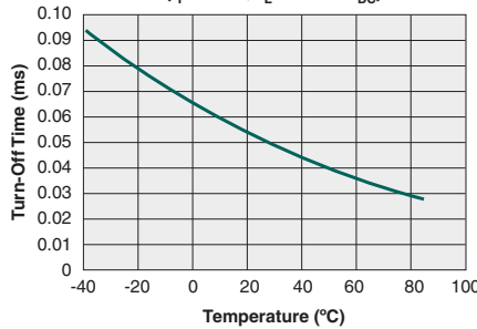
Typical Turn-Off Time vs. Temperature ( I_F=5\text{mA}, I_L=150\text{mA}_{DC} )
