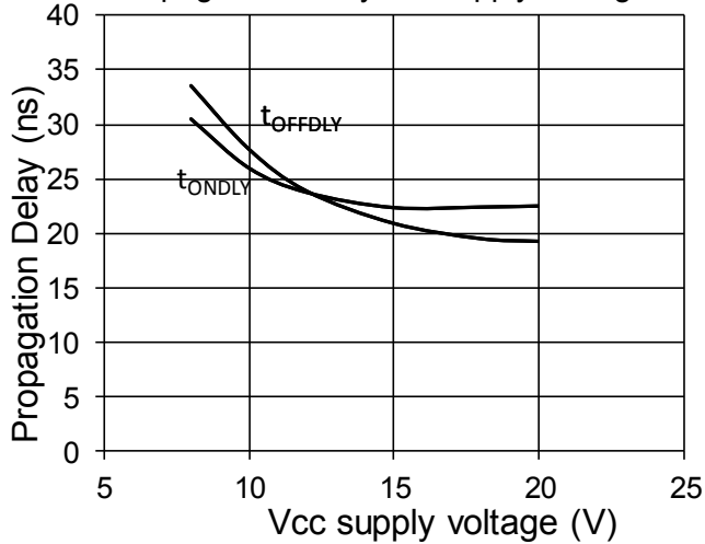
Fig. 6 Propagation Delay vs. Supply Voltage
