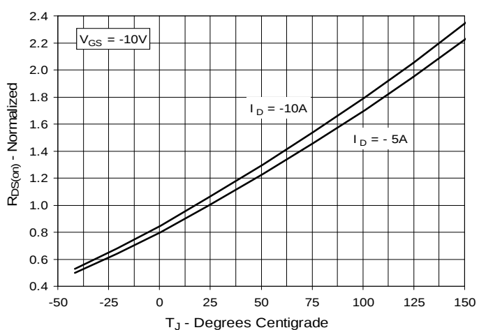
Fig. 4. R_{DS(on)} Normalized to I_D = -5A vs. Junction Temperature
