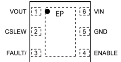
6-Pin MLF ® (ML) (Top View) MIC20X5
