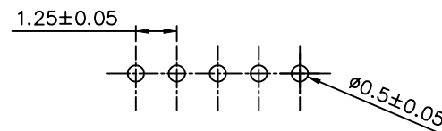
Recommended P.C.B Layout (Top Side) (Tolerance=±0.05)
