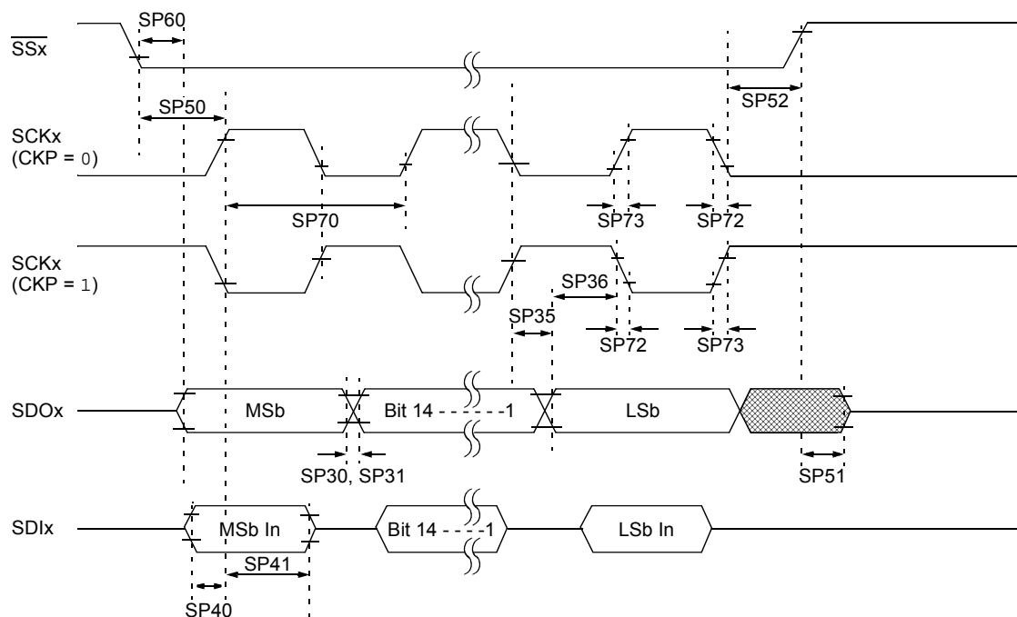
FIGURE 26-15: SPIx SLAVE MODE (FULL-DUPLEX, CKP = 1, CKP = 0, SMP = 0) TIMING CHARACTERISTICS
