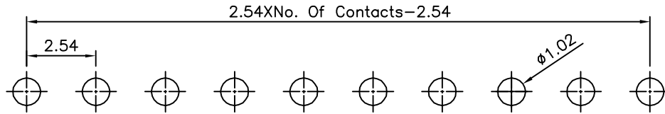
Recommended P.C.B. Layout(Top View) (PCB Board Tolerance±0.05)
