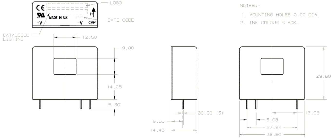
Mounting Dimensions - for reference only (mm)
