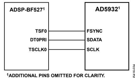
Figure 34. ADSP-BF527 to AD5932 Interface
